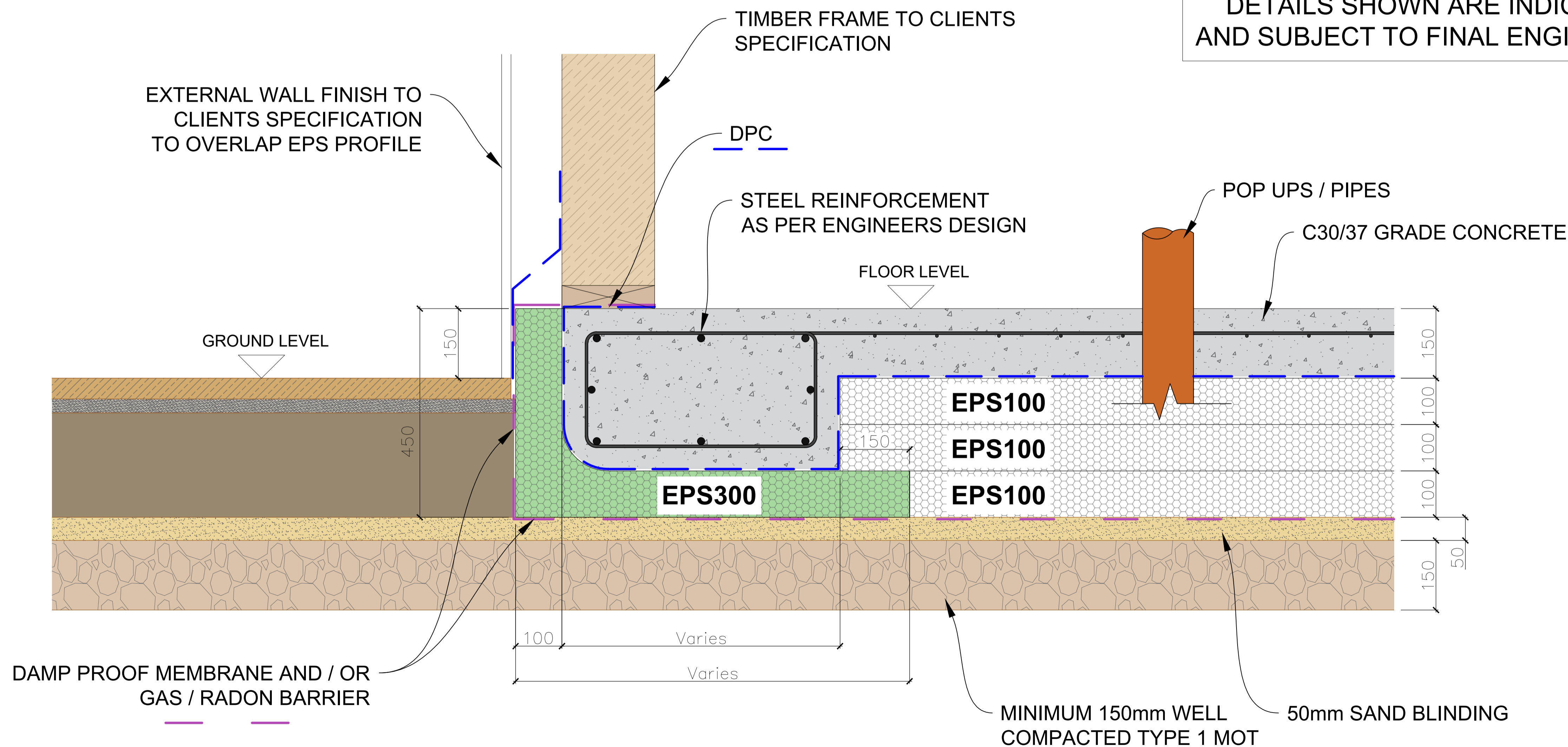
TYPICAL TIMBER FRAME EDGE SECTION - AFTER CONCRETE POUR
