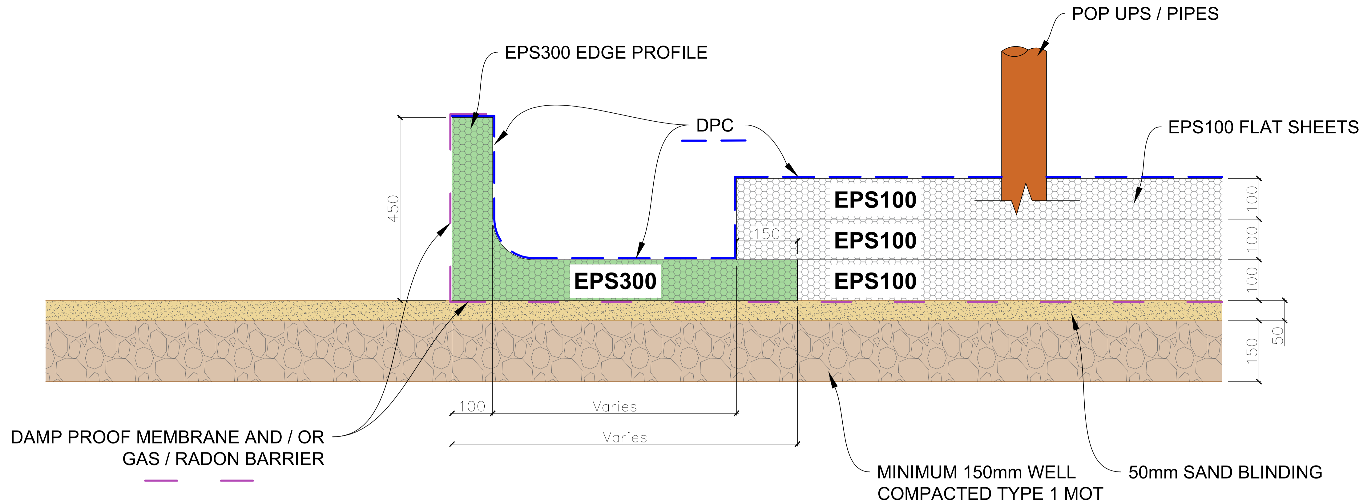
TYPICAL TIMBER FRAME EDGE SECTION - BEFORE CONCRETE POUR
