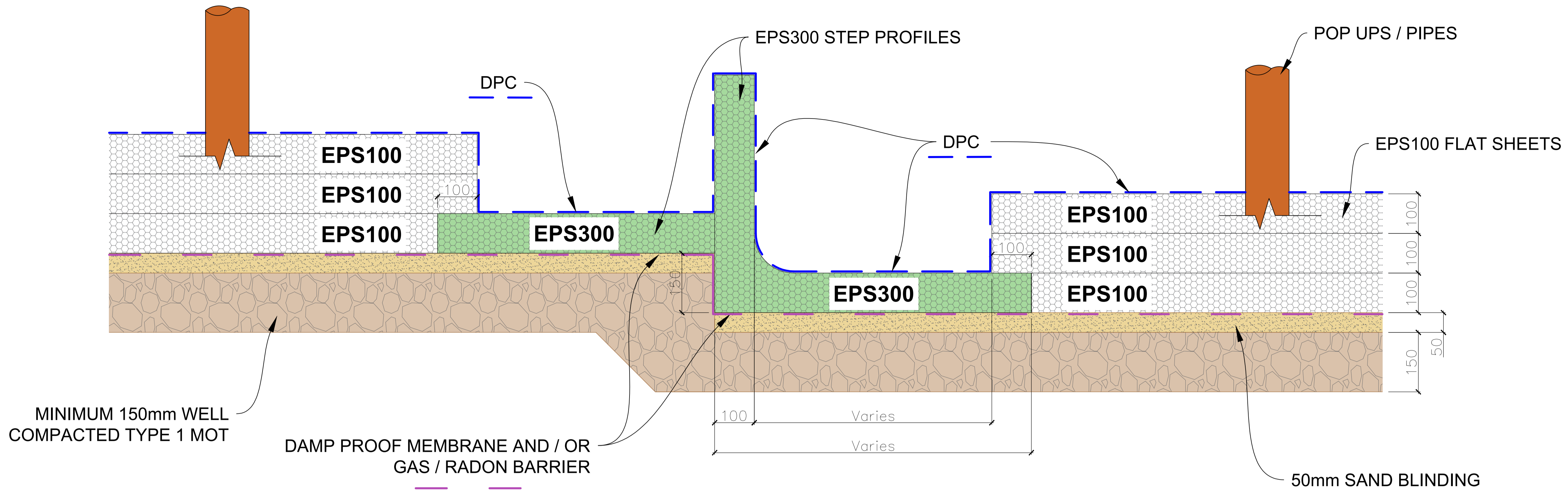
TYPICAL STEPPED FOUNDATION - BEFORE CONCRETE POUR
