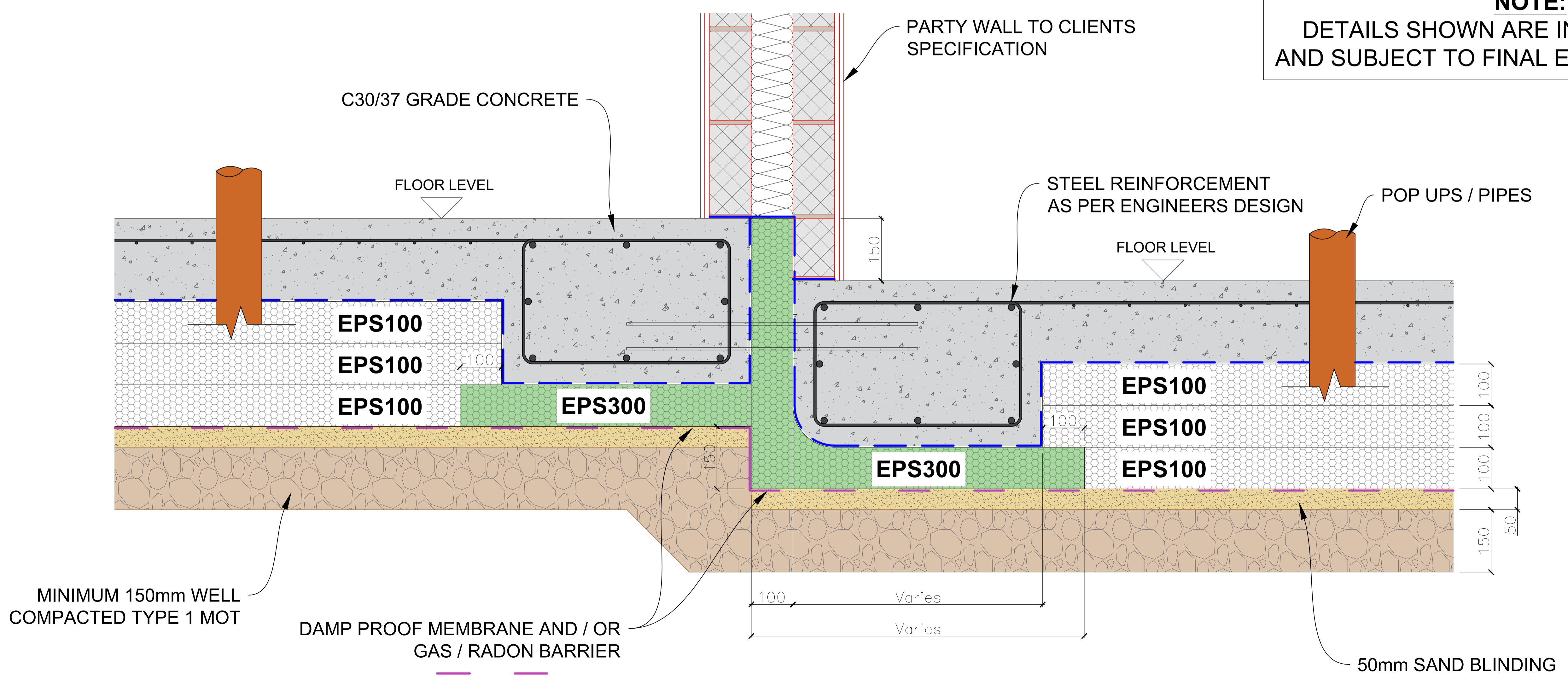
TYPICAL STEPPED FOUNDATION - AFTER CONCRETE POUR
