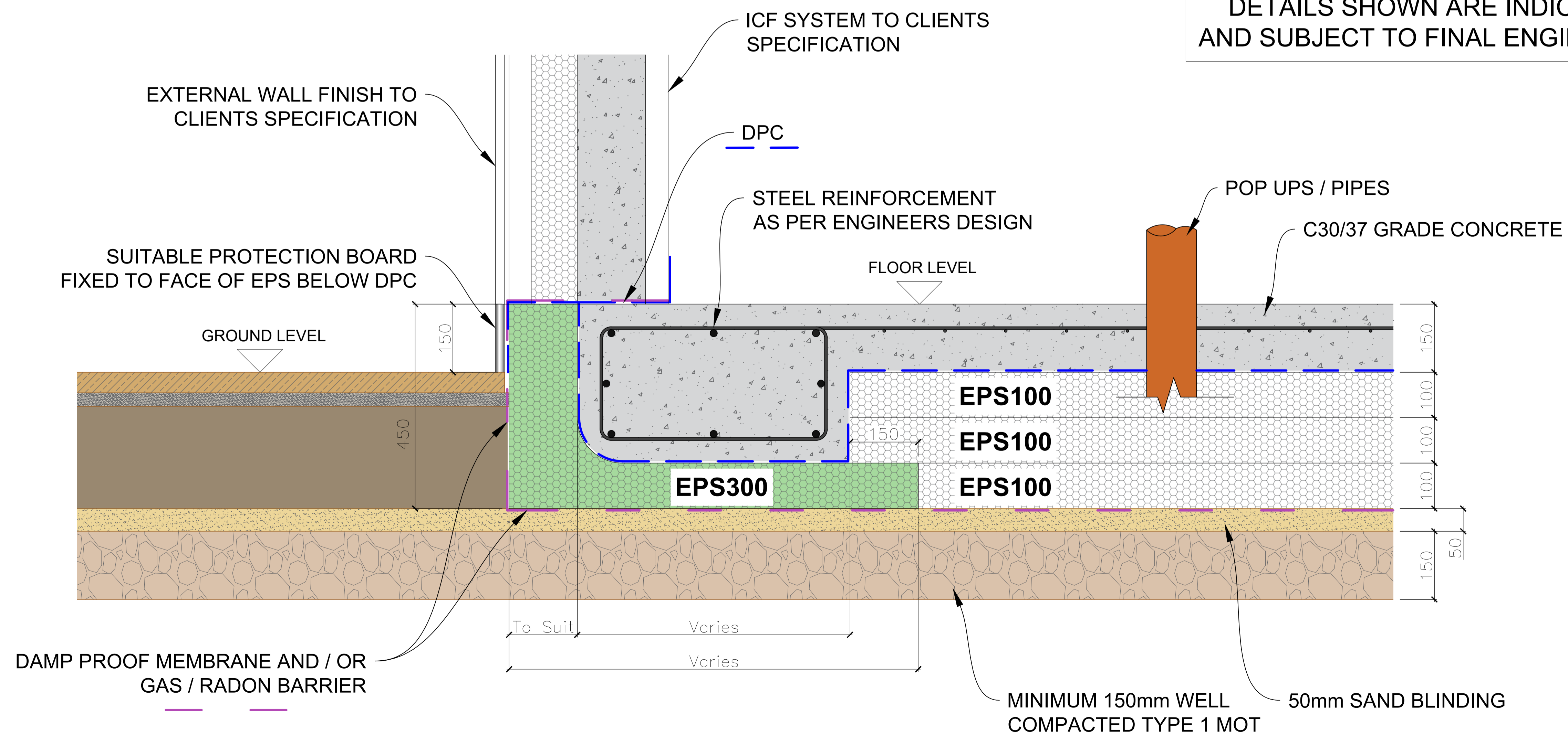
TYPICAL ICF WALL EDGE SECTION - AFTER CONCRETE POUR
